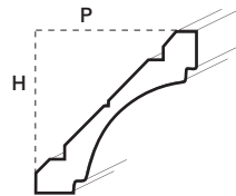
COVE RCRMC Height: 3⅛" Projection: 3⅛"
